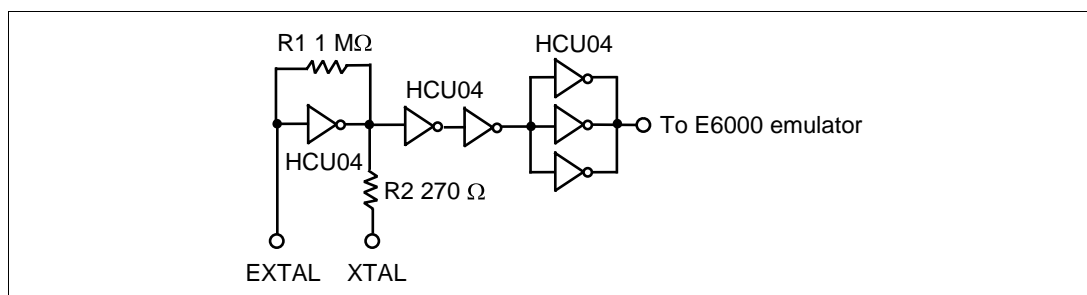
Figure 11 Oscillator Circuit
