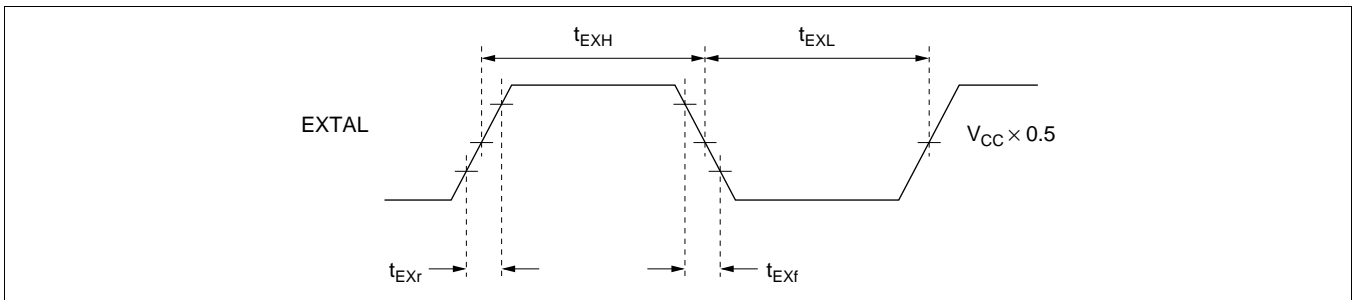
Figure 20-6 External Clock Input Timing
