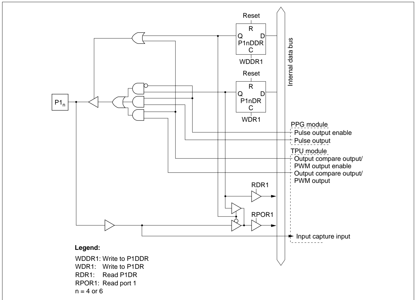
Figure C-1 (c) Port 1 Block Diagram (Pins P1 4 and P1 6 )
