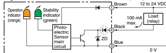
Protection for NPN output models
