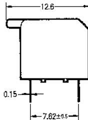
Side Actuated (long-lever)
