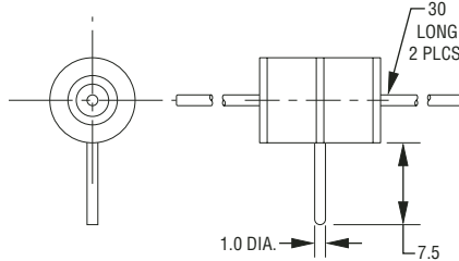
2026-XX-CB 0.8 mm dia. lead wire
