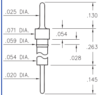
8859-0-00-XX-00-00-03-0 Press-fit in .056 mounting hole
