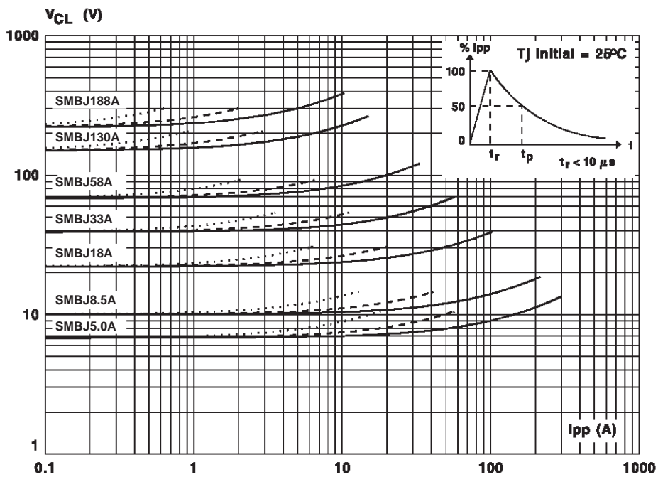
Fig. 3 : Clamping voltage versus peak pulse current. Exponential waveform t_p = 20 \mu s _____ t_p = 1 ms - - - - - t_p = 10 ms ..... T J Initial = 25°C
