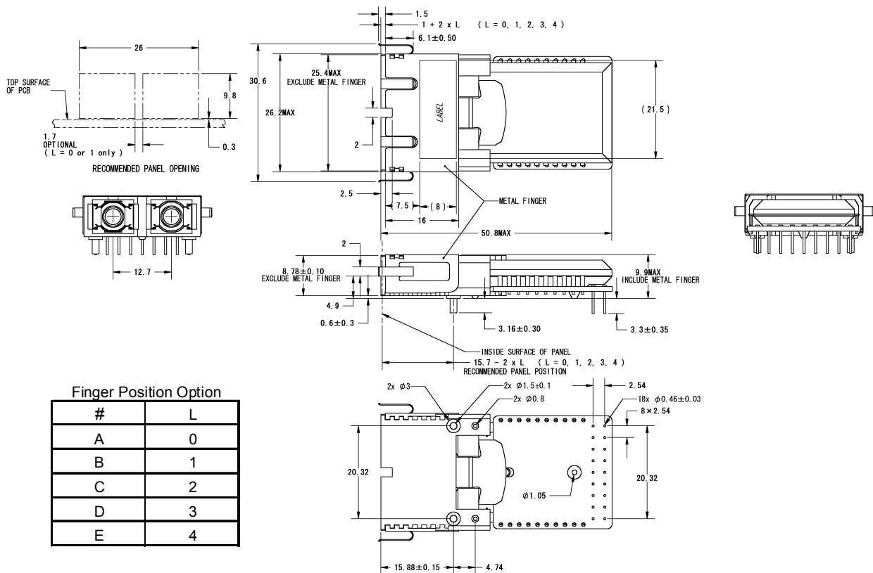
Figure2-3. Outline Dimensions (SCM7302-GC-#N / SCM7302-GC-#W)
