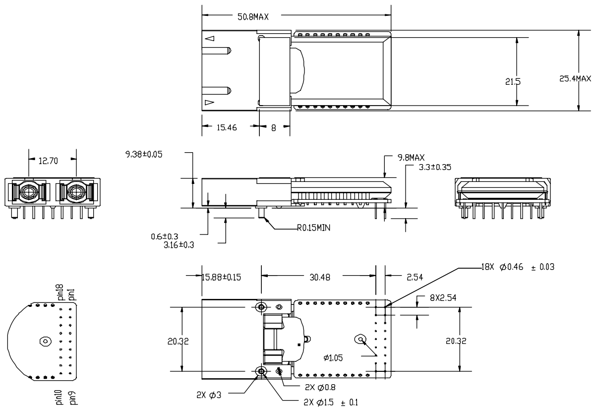
Figure2-1. Outline Dimensions(SCM7302-XC)
