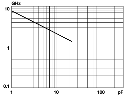
Typical Self Resonant Frequency vs. Capacitance Accu-F®/Accu-P® 0603
