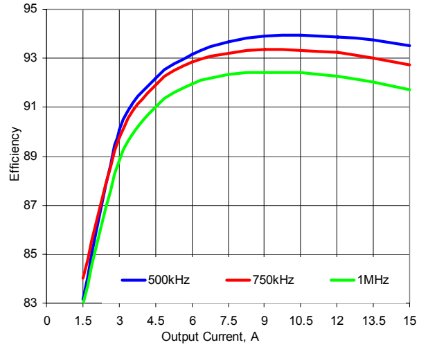
Figure 9. Efficiency vs. Load. V in =12V, V out =5V
