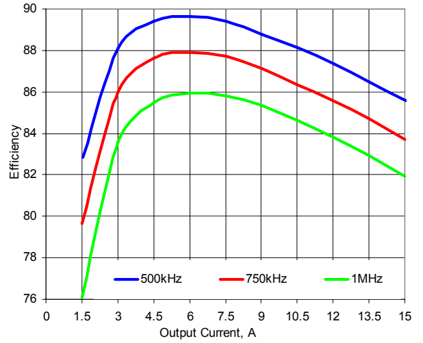
Figure 8. Efficiency vs. Load. V in =5V, V out =1.2V
