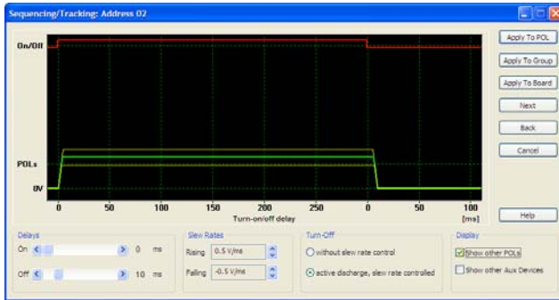
Figure 33. Sequencing/Tracking Window
