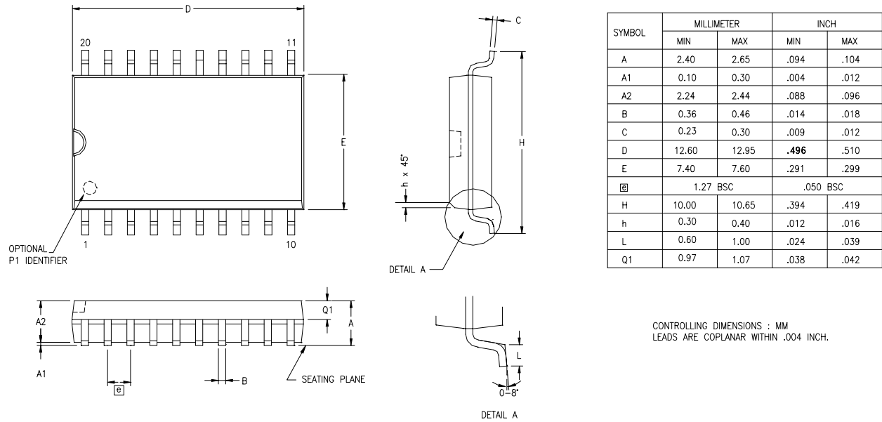
Figure 38. 20-Pin Small Outline Integrated Circuit (SOIC) Package
