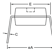
Figure 39. 20-Pin Plastic Dual In-line Package (PDIP)
