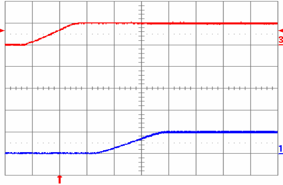
Fig. 1.0V.5: Turn-on transient for V_{out} = 1.0 V with application of V_{in} at full rated load current (resistive) and 47 \mu\text{F} external capacitance at V_{in} = 5 V. Top trace: V_{in} (5 V/div.); Bottom trace: output voltage (1 V/div.); Time scale: 2 ms/div.
