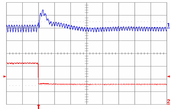
Fig. 3.3V.8: Output voltage response for V_{out} = 3.3 V to negative load current step change from 5 A to 2.5 A with slew rate of -5 A/ \mu\text{s} at V_{in} = 5 V. Top trace: output voltage (100 mV/div.); Bottom trace: load current (2 A/div.). C_o = 47 \mu\text{F} ceramic + 1 \mu\text{F} ceramic. Time scale: 20 \mu\text{s} /div.
