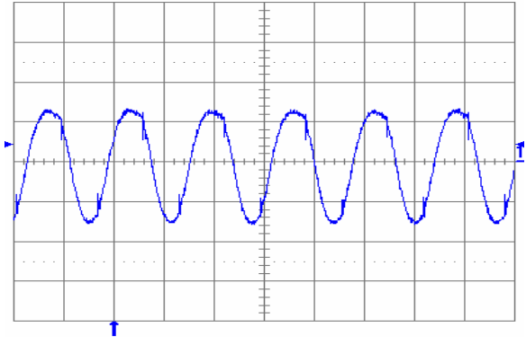
Fig. 2.5V.5: Output voltage ripple (20 mV/div.) at full rated load current into a resistive load with external capacitance 10 \mu\text{F} ceramic + 1 \mu\text{F} ceramic and V_{in} = 5 V for V_{out} = 2.5 V. Time scale: 2 \mu\text{s} /div.
