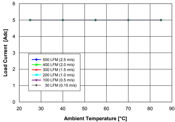
Fig. 2.5V.1: Available load current vs. ambient temperature and airflow rates for V_{out} = 2.5 V converter mounted vertically with V_{in} = 5 V, air flowing from pin 5 to pin 1 and maximum MOSFET temperature \leq 120 °C.
