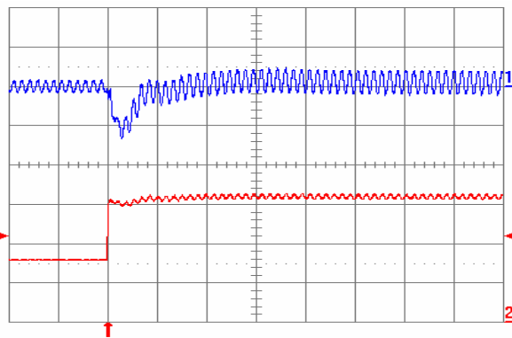
Fig. 2.0V.7: Output voltage response for V_{out} = 2.0 V to positive load current step change from 2.5 A to 5 A with slew rate of 5 \text{ A}/\mu\text{s} at V_{in} = 5 V. Top trace: output voltage (100 mV/div.); Bottom trace: load current (2 A/div.). C_o = 47 \mu\text{F} ceramic + 1 \mu\text{F} ceramic. Time scale: 20 \mu\text{s} /div.
