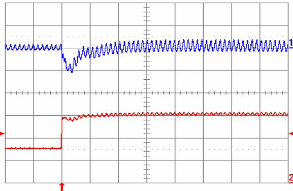
Fig. 1.2V.7: Output voltage response for V_{out} = 1.2\text{ V} to positive load current step change from 2.5\text{ A} to 5\text{ A} with slew rate of 5\text{ A}/\mu\text{s} at V_{in} = 5\text{ V} . Top trace: output voltage ( 100\text{ mV/div.} ); Bottom trace: load current ( 2\text{ A/div.} ). C_o = 47\ \mu\text{F} ceramic + 1\ \mu\text{F} ceramic. Time scale: 20\ \mu\text{s/div.}
