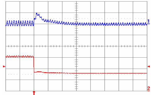
Fig. 1.0V.8: Output voltage response for V_{out} = 1.0 V to negative load current step change from 5 A to 2.5 A with slew rate of -5 A/ \mu\text{s} at V_{in} = 5 V. Top trace: output voltage (100 mV/div.); Bottom trace: load current (2 A/div.). C_o = 47 \mu\text{F} ceramic + 1 \mu\text{F} ceramic. Time scale: 20 \mu\text{s} /div.
