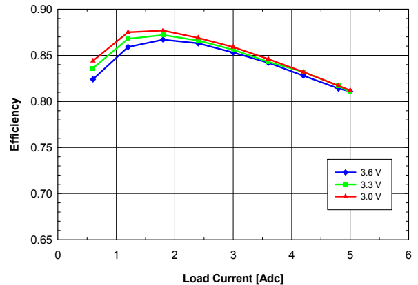
Fig. 0.7525V.4: Efficiency vs. load current and input voltage for V_{out} = 0.7525\text{ V} converter mounted vertically with air flowing from pin 5 to pin 1 at a rate of 200 LFM (1 m/s) and T_a = 25\text{ }^{\circ}\text{C} .
