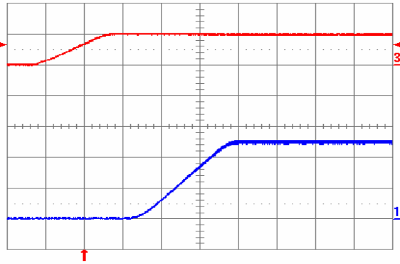
Fig. 2.5V.4: Turn-on transient for V_{out} = 2.5 V with application of V_{in} at full rated load current (resistive) and 47 \mu\text{F} external capacitance at V_{in} = 5 V. Top trace: V_{in} (5 V/div.); Bottom trace: output voltage (1V/div.); Time scale: 2 ms/div.
