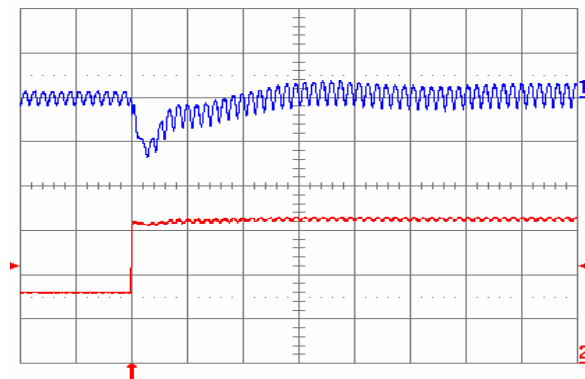
Fig. 3.3V.7: Output voltage response for V_{out} = 3.3 V to positive load current step change from 2.5 A to 5 A with slew rate of 5 A/ \mu\text{s} at V_{in} = 5 V. Top trace: output voltage (100 mV/div.); Bottom trace: load current (2 A/div.). C_o = 47 \mu\text{F} ceramic + 1 \mu\text{F} ceramic. Time scale: 20 \mu\text{s} /div.
