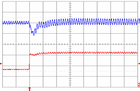
Fig. 1.5V.7: Output voltage response for V_{out} = 1.5 V to positive load current step change from 2.5 A to 5 A with slew rate of 5 A/ \mu s at V_{in} = 5 V. Top trace: output voltage (100 mV/div.); Bottom trace: load current (2 A/div.). C_o = 47 \mu F ceramic + 1 \mu F ceramic. Time scale: 20 \mu s/div.
