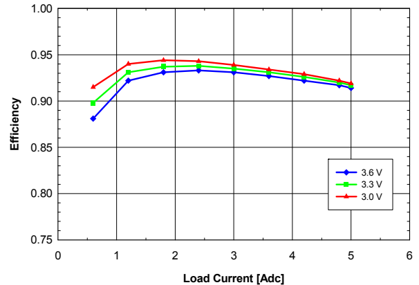
Fig. 2.0V.4: Efficiency vs. load current and input voltage for V_{out} = 2.0\text{ V} converter mounted horizontally with air flowing from pin 5 to pin 1 at a rate of 200 LFM (1 m/s) and T_a = 25\text{ }^{\circ}\text{C} .
