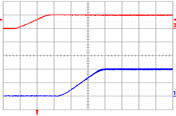
Fig. 2.0V.5: Turn-on transient for V_{out} = 2.0 V with application of V_{in} at full rated load current (resistive) and 47 \mu\text{F} external capacitance at V_{in} = 5 V. Top trace: V_{in} (5 V/div.); Bottom trace: output voltage (1 V/div.); Time scale: 2 ms/div.
