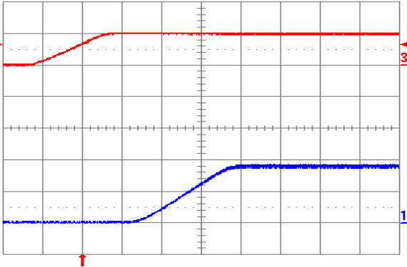
Fig. 1.8V.5: Turn-on transient for V_{out} = 1.8\text{ V} with application of V_{in} at full rated load current (resistive) and 47\text{ }\mu\text{F} external capacitance at V_{in} = 5\text{ V} . Top trace: V_{in} ( 5\text{ V/div.} ); Bottom trace: output voltage ( 1\text{ V/div.} ); Time scale: 2\text{ ms/div.}
