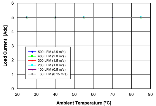
Fig. 2.5V.2: Available load current vs. ambient temperature and airflow rates for V_{out} = 2.5 V converter mounted horizontally with V_{in} = 5 V, air flowing from pin 5 to pin 1 and maximum MOSFET temperature \leq 120 °C.
