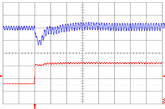
Fig. 2.5V.7: Output voltage response for V_{out} = 2.5 V to positive load current step change from 2.5 A to 5 A with slew rate of 5 \text{ A}/\mu\text{s} at V_{in} = 5 V. Top trace: output voltage (100 mV/div.); Bottom trace: load current (2 A/div.). C_o = 47 \mu\text{F} ceramic + 1 \mu\text{F} ceramic. Time scale: 20 \mu\text{s} /div.
