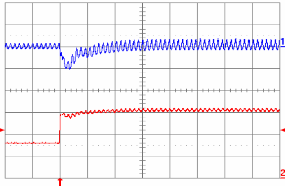
Fig. 1.0V.7: Output voltage response for V_{out} = 1.0 V to positive load current step change from 2.5 A to 5 A with slew rate of 5 A/ \mu\text{s} at V_{in} = 5 V. Top trace: output voltage (100 mV/div.); Bottom trace: load current (2 A/div.). C_o = 47 \mu\text{F} ceramic + 1 \mu\text{F} ceramic. Time scale: 20 \mu\text{s} /div.
