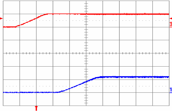
Fig. 1.2V.5: Turn-on transient for V_{out} = 1.2\text{ V} with application of V_{in} at full rated load current (resistive) and 47\ \mu\text{F} external capacitance at V_{in} = 5\text{ V} . Top trace: V_{in} ( 5\text{ V/div.} ); Bottom trace: output voltage ( 1\text{ V/div.} ); Time scale: 2\text{ ms/div.}
