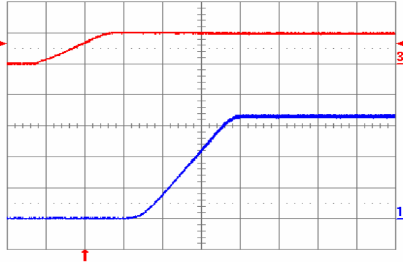
Fig. 3.3V.5: Turn-on transient for V_{out} = 3.3 V with application of V_{in} at full rated load current (resistive) and 47 \mu\text{F} external capacitance at V_{in} = 5 V. Top trace: V_{in} (5 V/div.); Bottom trace: output voltage (1V/div.); Time scale: 2 ms/div.
