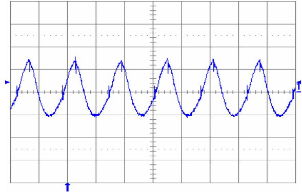
Fig. 1.2V.6: Output voltage ripple ( 20\text{ mV/div.} ) at full rated load current into a resistive load with external capacitance 10\ \mu\text{F} ceramic + 1\ \mu\text{F} ceramic and V_{in} = 5\text{ V} for V_{out} = 1.2\text{ V} . Time scale: 2\ \mu\text{s/div.}
