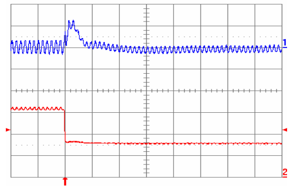
Fig. 2.0V.8: Output voltage response for V_{out} = 2.0 V to negative load current step change from 5 A to 2.5 A with slew rate of -5 \text{ A}/\mu\text{s} at V_{in} = 5 V. Top trace: output voltage (100 mV/div.); Bottom trace: load current (2 A/div.). C_o = 47 \mu\text{F} ceramic + 1 \mu\text{F} ceramic. Time scale: 20 \mu\text{s} /div.
