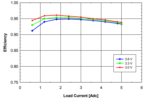
Fig. 2.5V.4: Efficiency vs. load current and input voltage for V_{out} = 2.5 V converter mounted vertically with air flowing from pin 5 to pin 1 at a rate of 200 LFM (1 m/s) and T_a = 25 °C.
