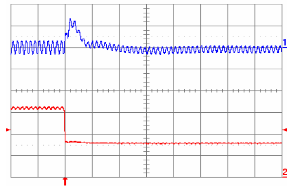
Fig. 2.5V.8: Output voltage response for V_{out} = 2.5 V to negative load current step change from 5 A to 2.5 A with slew rate of -5 \text{ A}/\mu\text{s} at V_{in} = 5 V. Top trace: output voltage (100 mV/div.); Bottom trace: load current (2 A/div.). C_o = 47 \mu\text{F} ceramic + 1 \mu\text{F} ceramic. Time scale: 20 \mu\text{s} /div.
