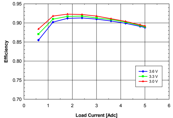
Fig. 1.5V.4: Efficiency vs. load current and input voltage for V_{out} = 1.5 V converter mounted vertically with air flowing from pin 5 to pin 1 at a rate of 200 LFM (1 m/s) and T_a = 25 °C.
