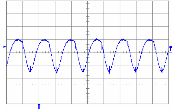
Fig. 3.3V.6: Output voltage ripple (20 mV/div.) at full rated load current into a resistive load with external capacitance 10 \mu\text{F} ceramic + 1 \mu\text{F} ceramic and V_{in} = 5 V for V_{out} = 3.3 V. Time scale: 2 \mu\text{s} /div.
