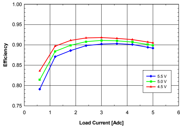
Fig. 2.0V.3: Efficiency vs. load current and input voltage for V_{out} = 2.0\text{ V} converter mounted vertically with air flowing from pin 5 to pin 1 at a rate of 200 LFM (1 m/s) and T_a = 25\text{ }^{\circ}\text{C} .
