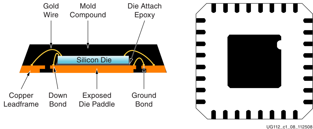
Figure 1-8: On the Left is the QFN Cross-Section. On the Right is the Bottom View.
