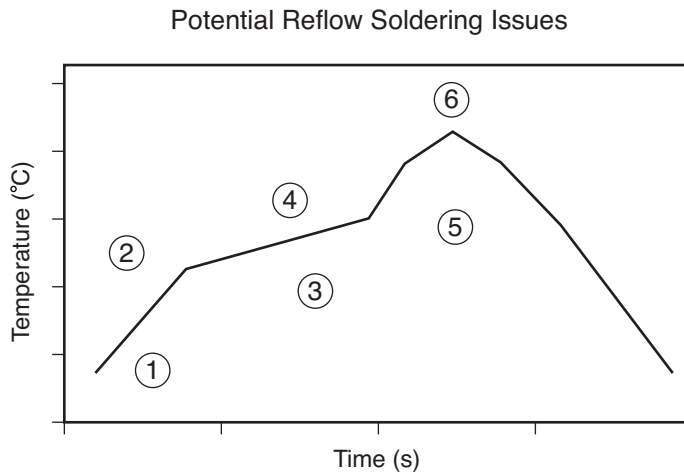
Figure 7-2: Soldering Problems Summary
