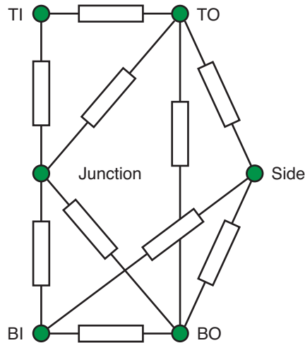
DELPHI BCI-CTM Topology for FCBGA
