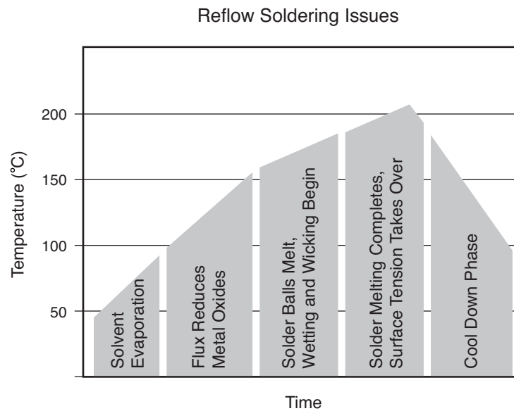
Figure 7-1: Soldering Sequence
