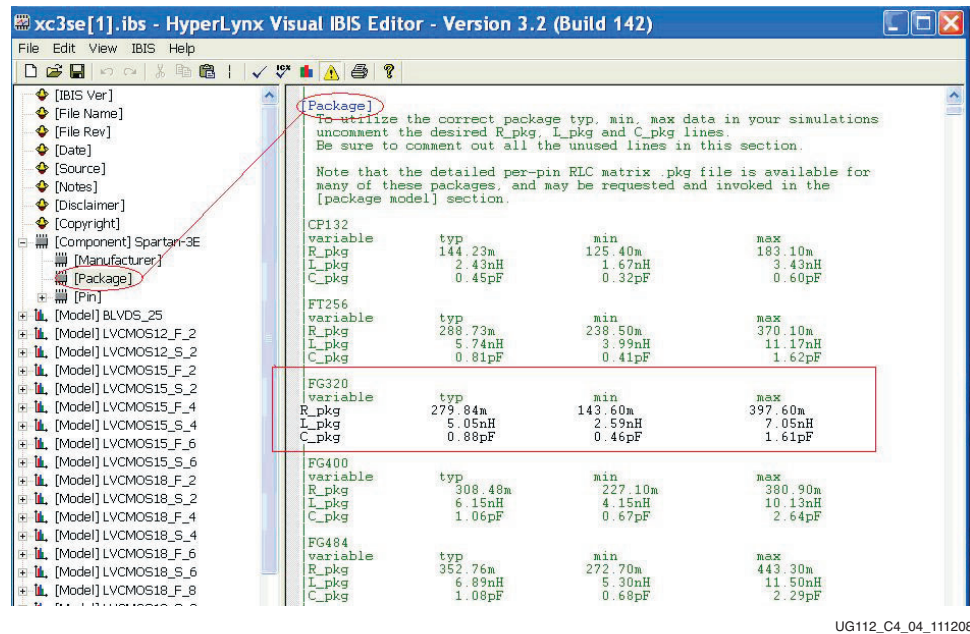
Figure 4-4: Embedded Electrical Parasitics Data
