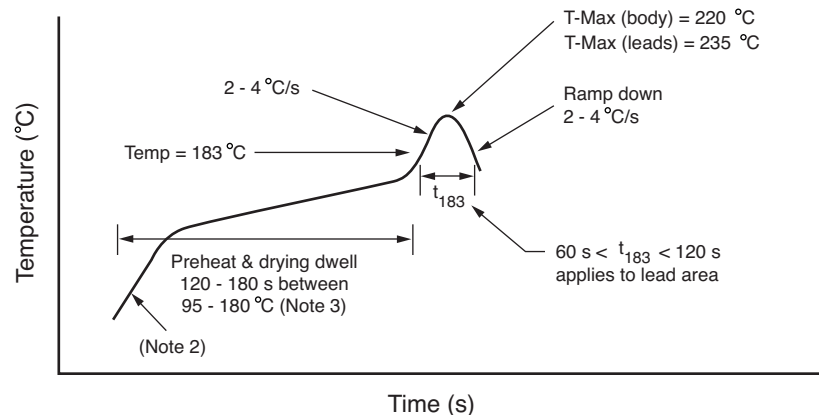
Figure 7-3: Typical Conditions for IR Reflow Soldering of Sn/Pb Solder
