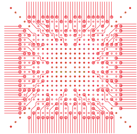
Second Signal Layer
