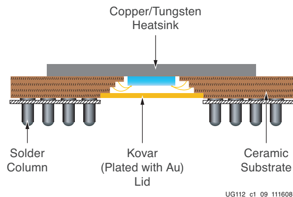
Figure 1-9: CG560 Package
