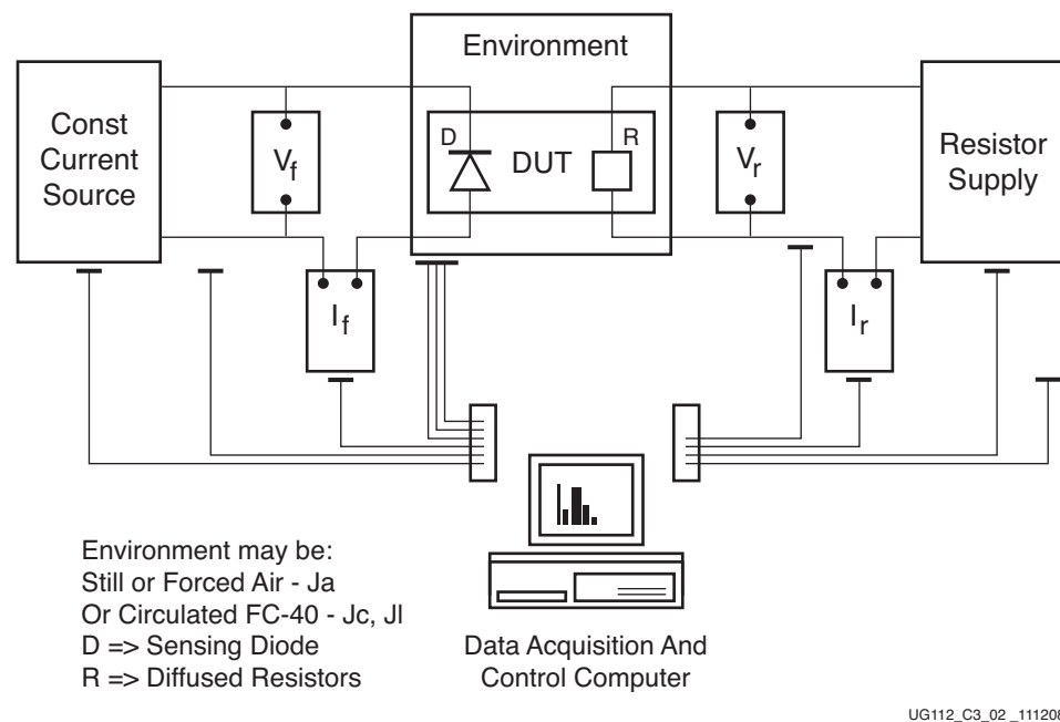
Figure 3-2: Thermal Measurement Setup (Schematic for Junction to Reference)
