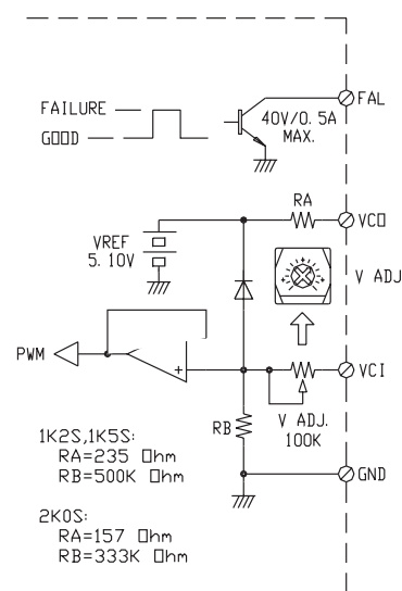
VCI AND VCO SIGNAL
