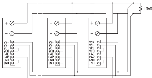
PARALLEL OPERATION WITH REMOTE SENSING
