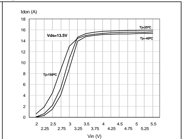
Figure 26. Transfer characteristics
