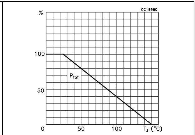
Figure 24. Derating curve
