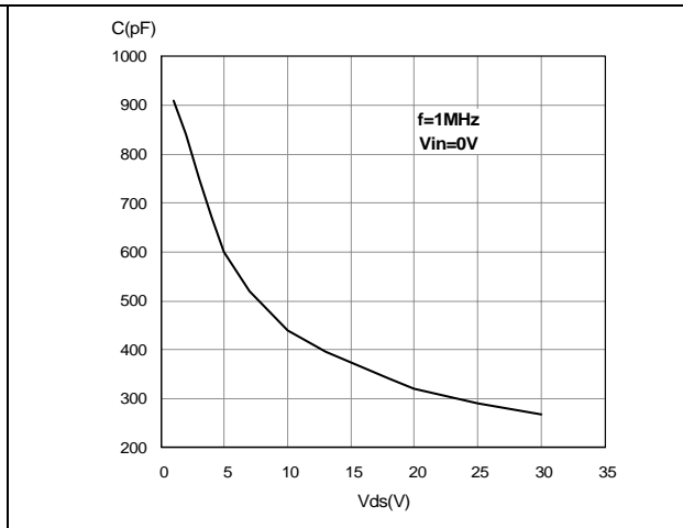
Figure 30. Capacitance variations
