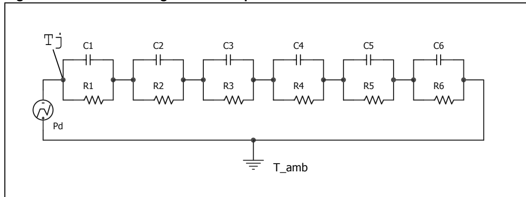
Figure 24. Thermal fitting model of a quad channel HSD in PowerSO-10
