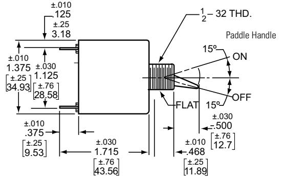
Two Pole, Toggle
