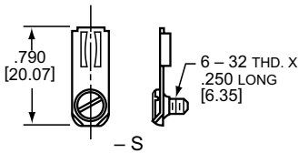
Screw Terminal Adapter (All Versions)
