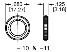
Knurled Nut
