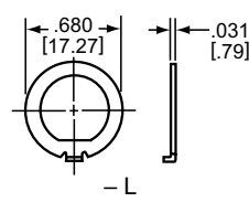
Locking Ring (Toggle)
